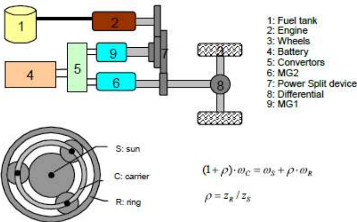
Combined HEV with planetary unit as used in the Toyota Prius
